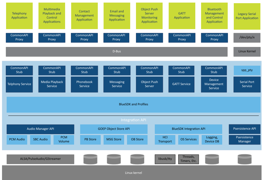
Fig.: Represents the daemon architecture with all core stack components and profiles running in the context of a user space Linux daemon.
